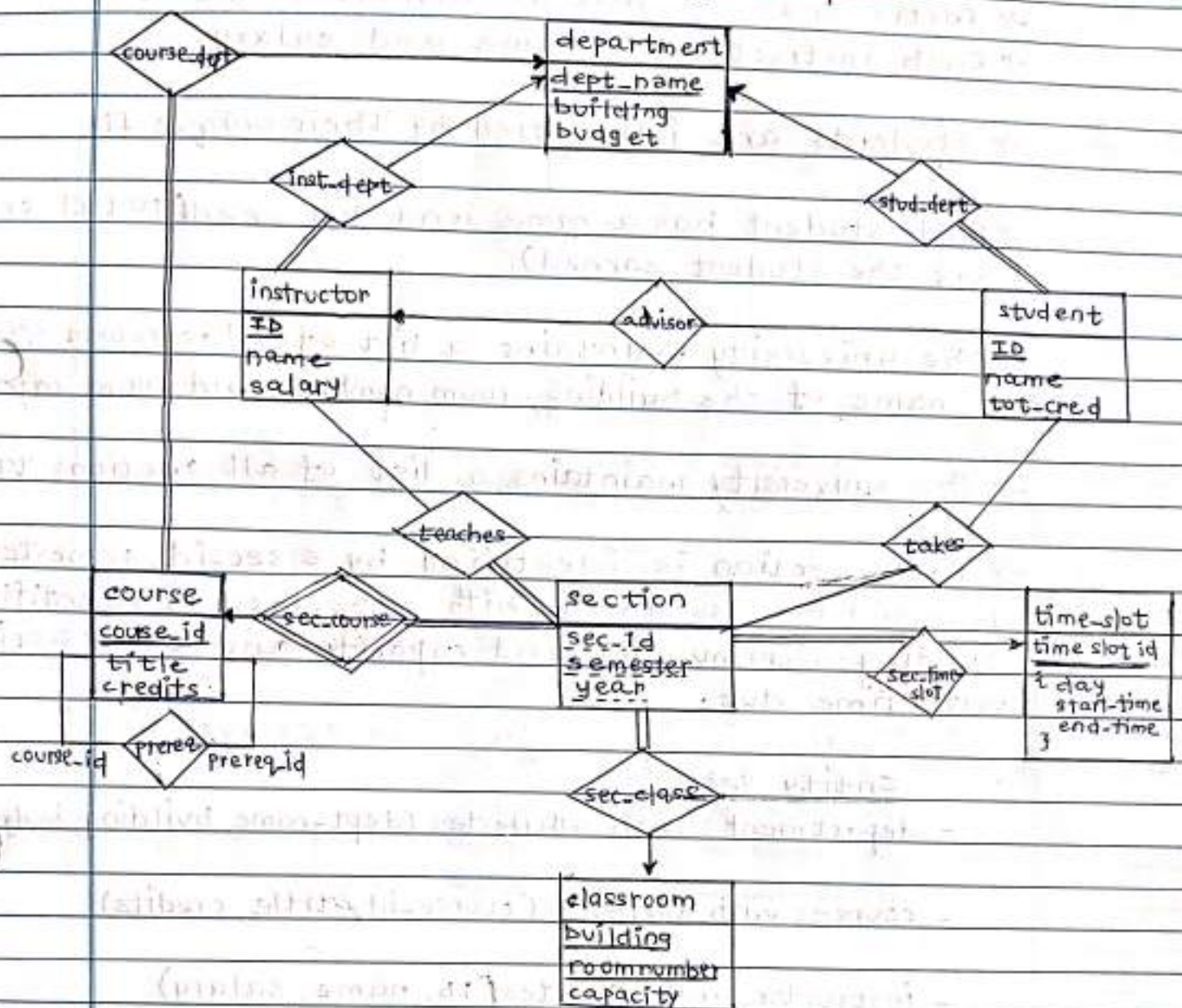
Fig 3: E-R Diagram for a University Enterprise
